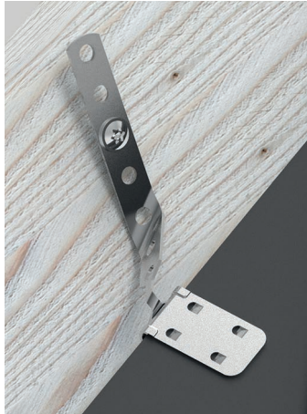
512 secures cut tile at the hip
