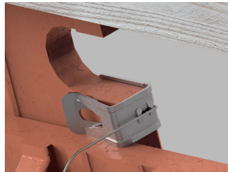
“Replacement lug” for beaver tail tiles Further the 513 can be used as a replacement lug. The 513 is hammered-in on the side so that the tile has a hold on the batten or sub-construction.
